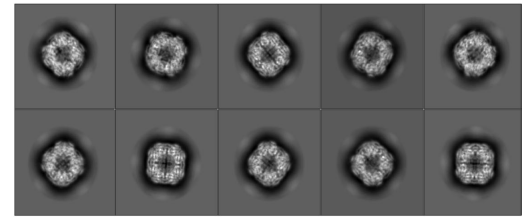
CryoEM
